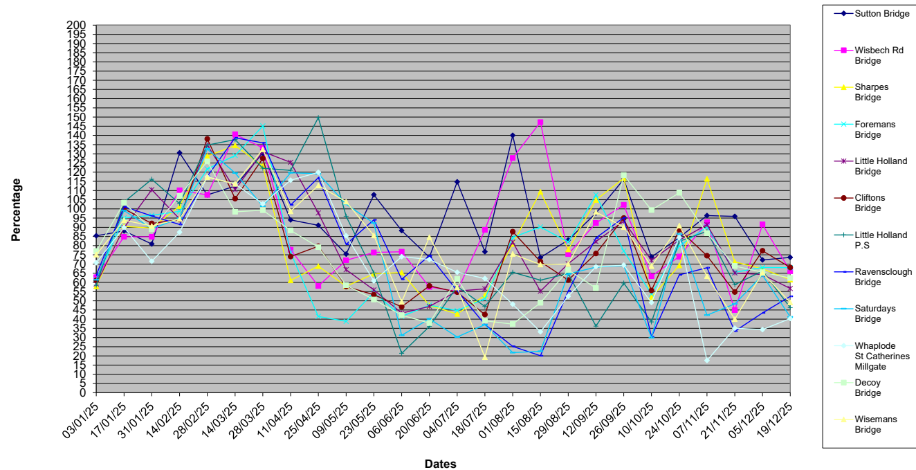
Dissolved Oxygen Near Bed
